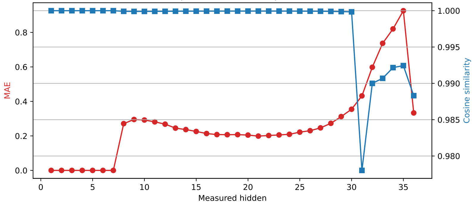
Qwen2.5-3B | Quantized layer 7 | float64 → int2
