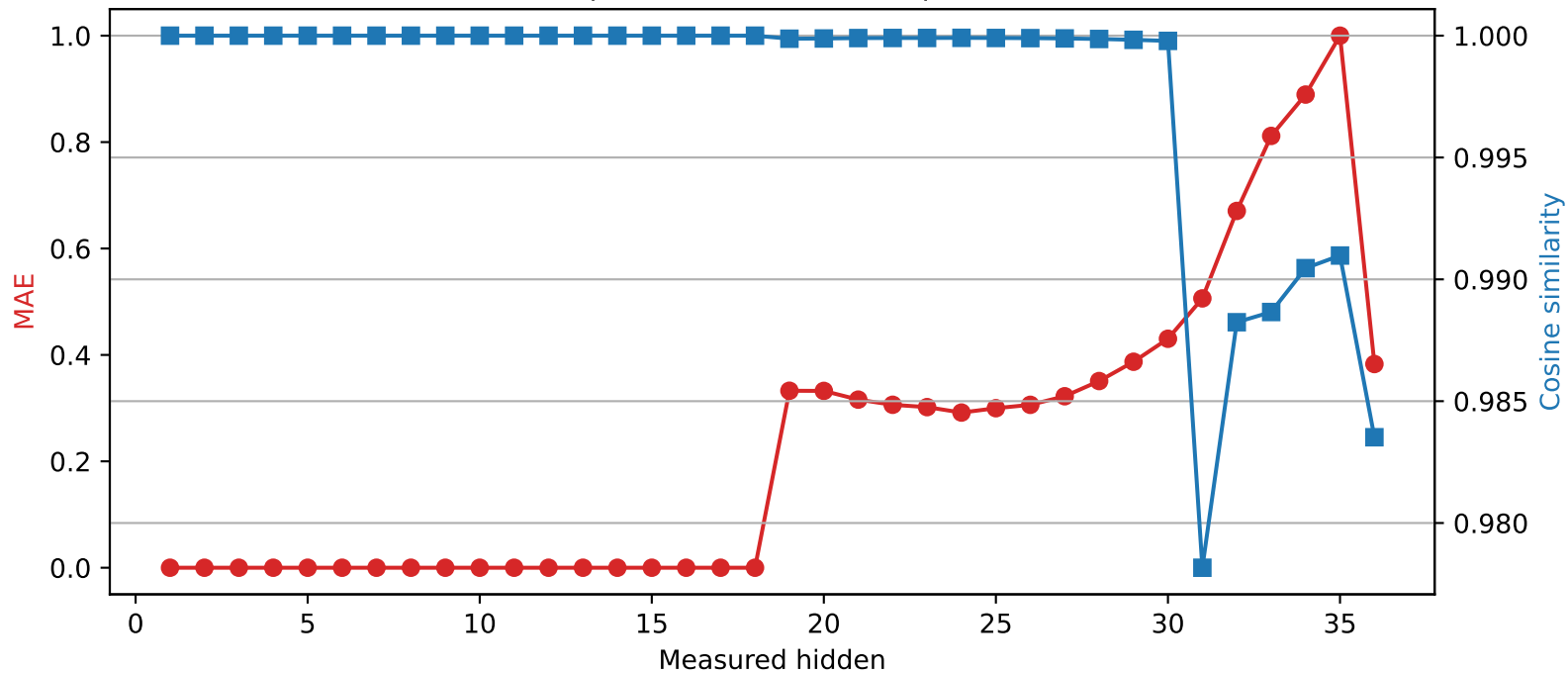
Qwen2.5-3B | Quantized layer 18 | float64 → int2
