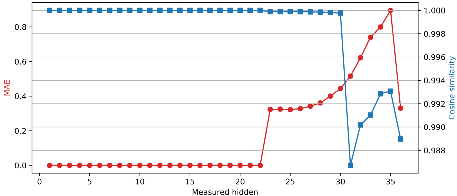
Qwen2.5-3B | Quantized layer 22 | float64 → int2
