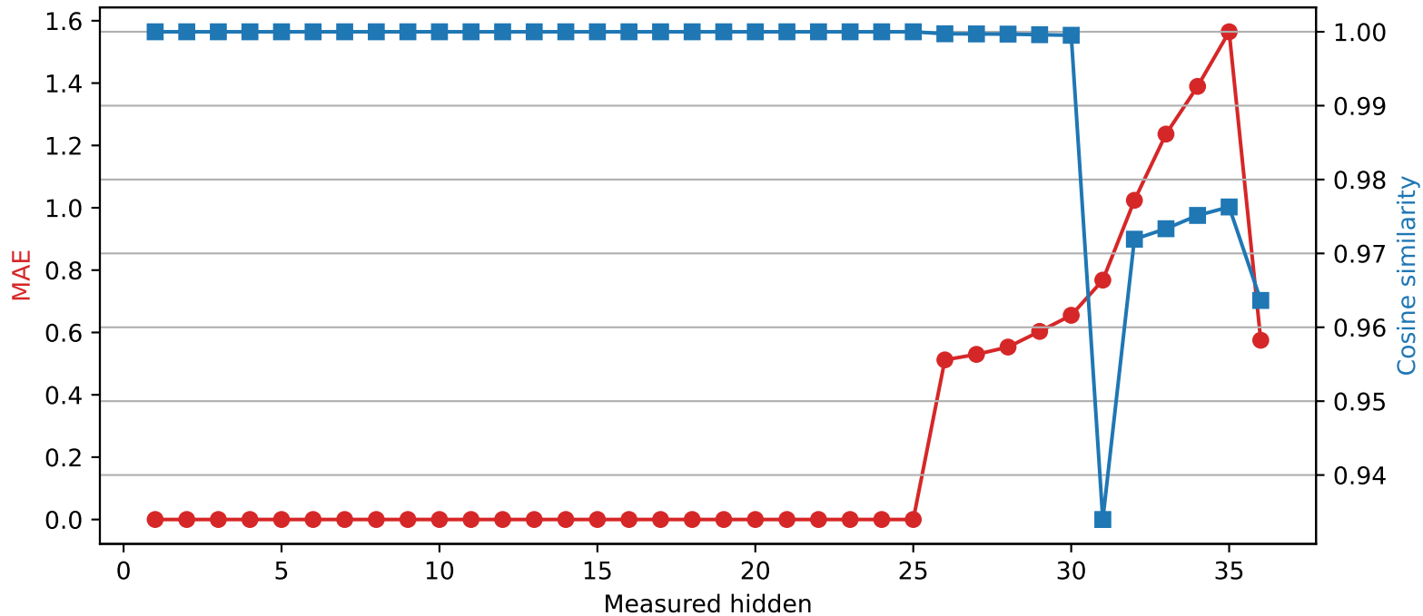
Qwen2.5-3B | Quantized layer 25 | float64 → int2
