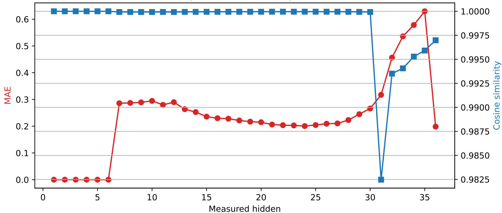
Qwen2.5-3B | Quantized layer 6 | float64 → int2
