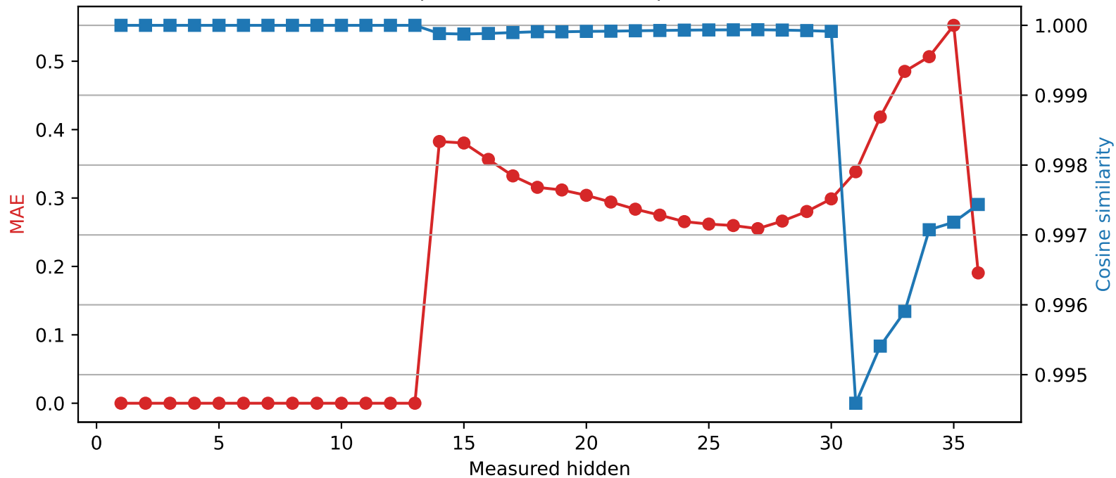
Qwen2.5-3B | Quantized layer 13 | float64 → int2
