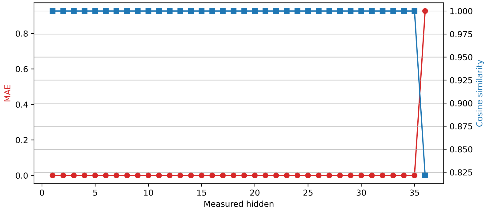
Qwen2.5-3B | Quantized layer 35 | float64 → int2
