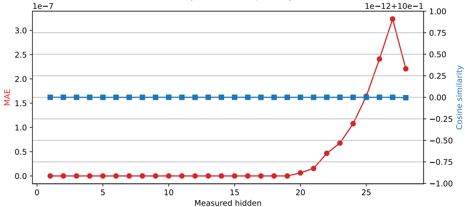
Qwen2.5-7B-Instruct | Quantized layer 19 | float64 → int32
