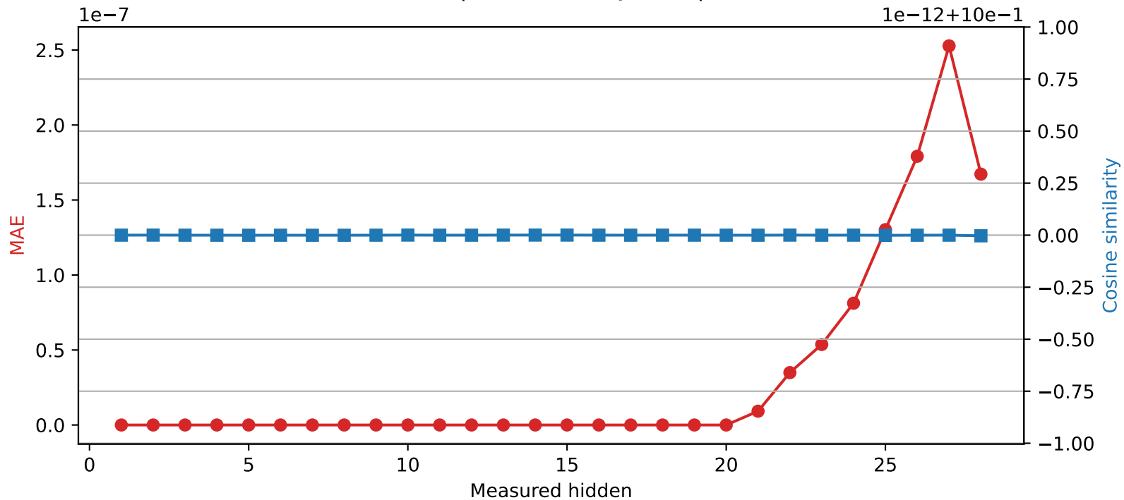
Qwen2.5-7B-Instruct | Quantized layer 20 | float64 → int32
