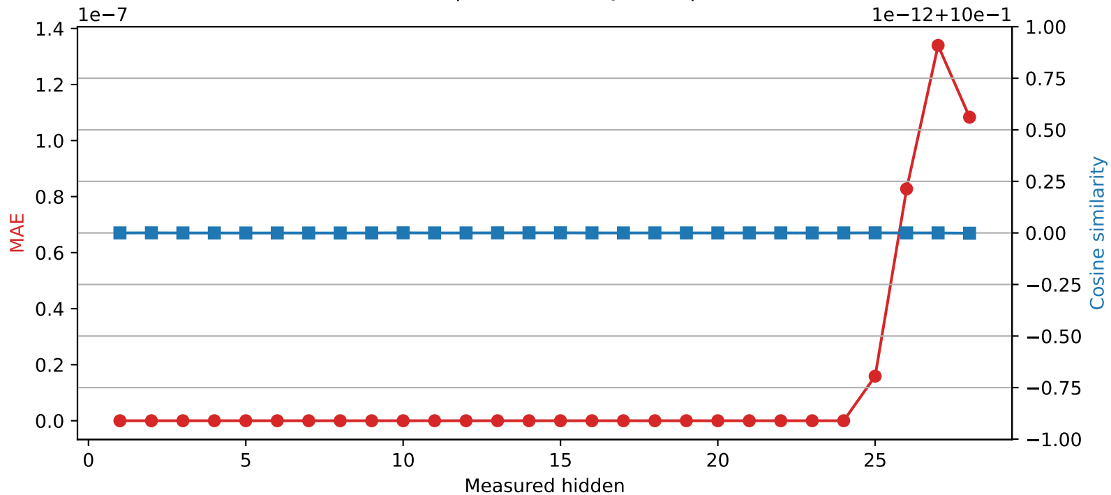
Qwen2.5-7B-Instruct | Quantized layer 24 | float64 → int32
