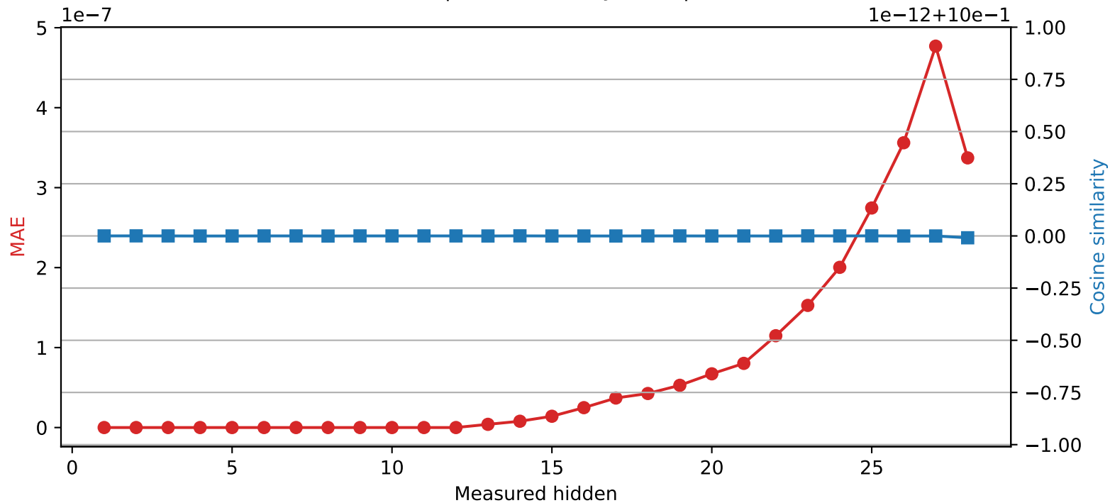
Qwen2.5-7B-Instruct | Quantized layer 12 | float64 → int32
