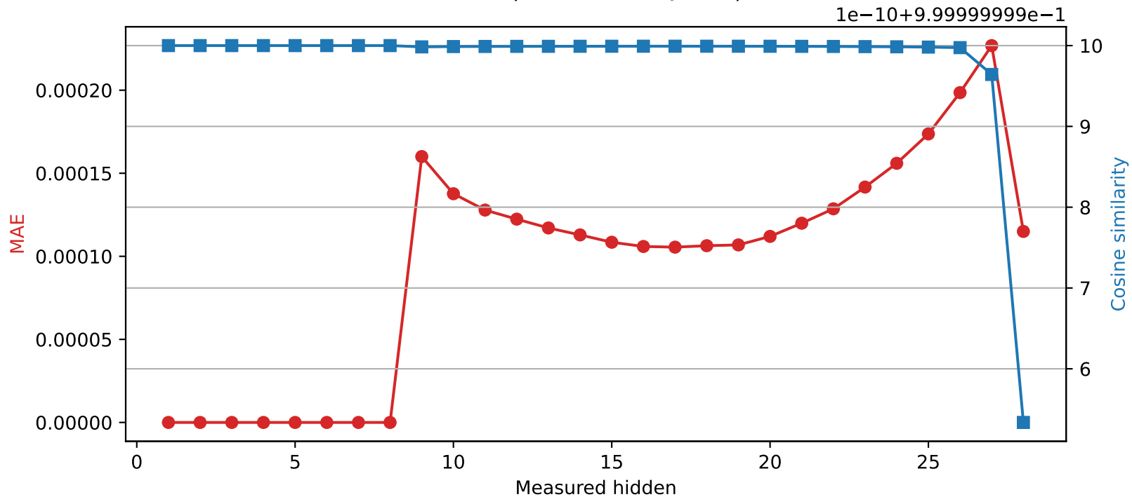
Qwen2.5-7B-Instruct | Quantized layer 8 | float32 → int16
