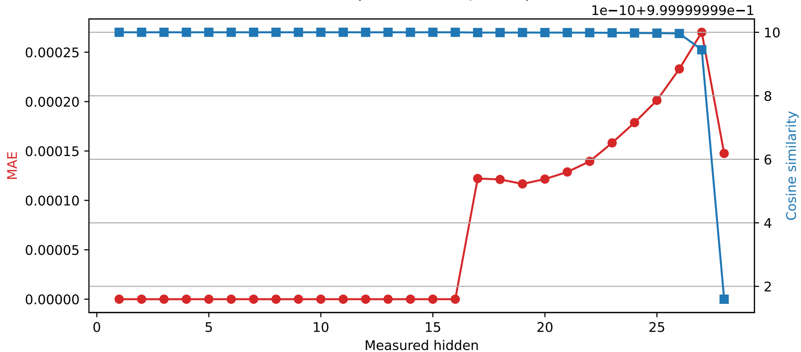
Qwen2.5-7B-Instruct | Quantized layer 16 | float32 \rightarrow int16
