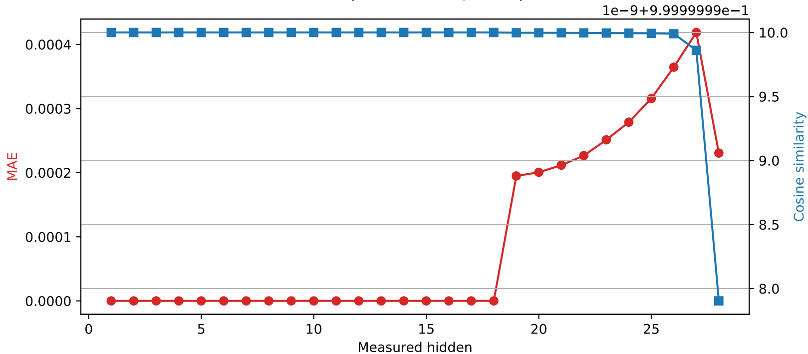
Qwen2.5-7B-Instruct | Quantized layer 18 | float32 → int16
