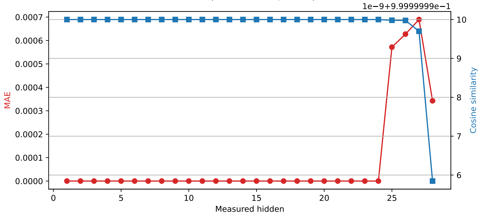
Qwen2.5-7B-Instruct | Quantized layer 24 | float32 \rightarrow int16
