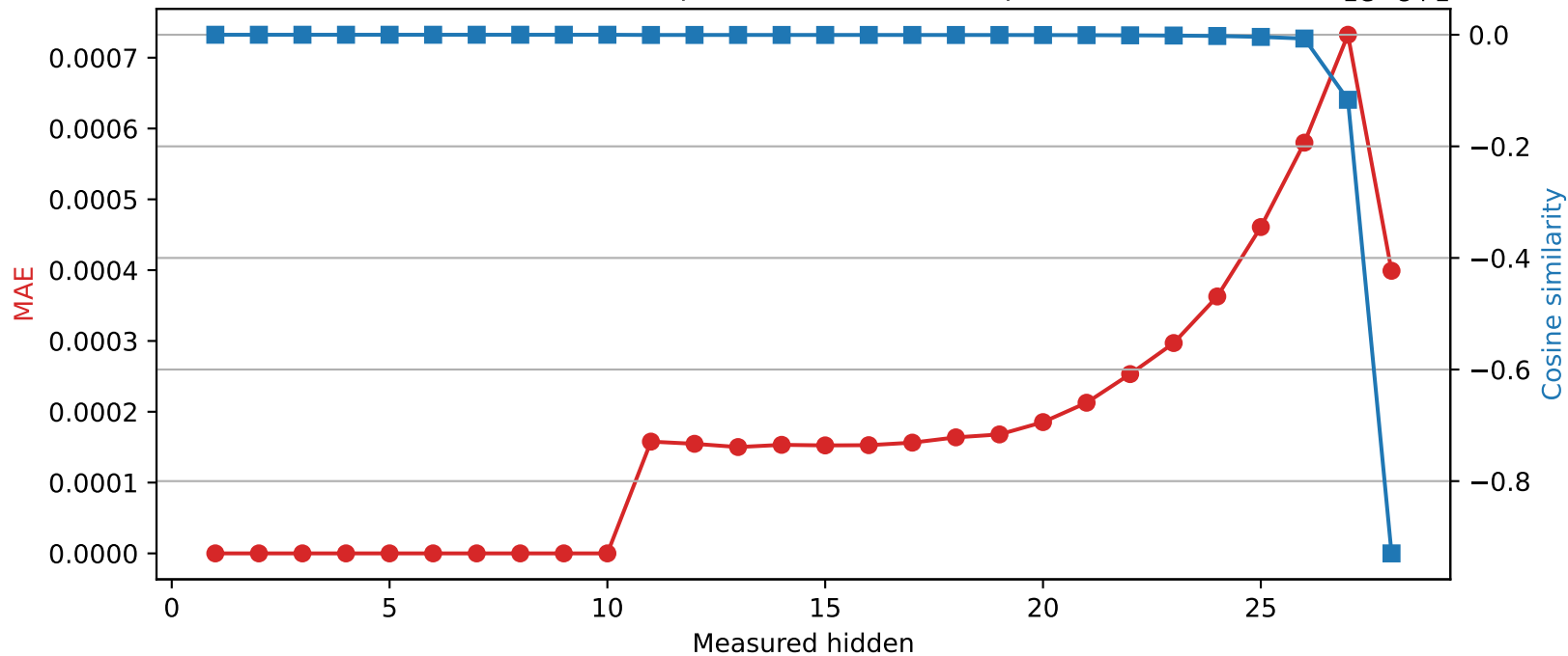
Qwen2.5-7B-Instruct | Quantized layer 10 | float32 → int16
