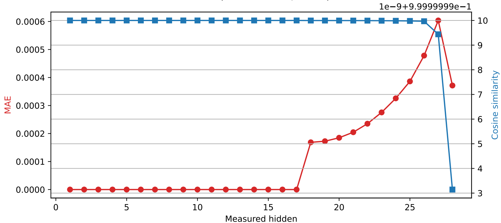
Qwen2.5-7B-Instruct | Quantized layer 17 | float32 → int16
