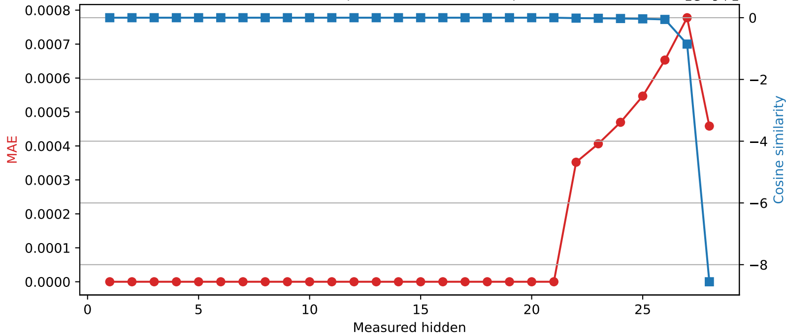
Qwen2.5-7B-Instruct | Quantized layer 21 | float32 → int16
