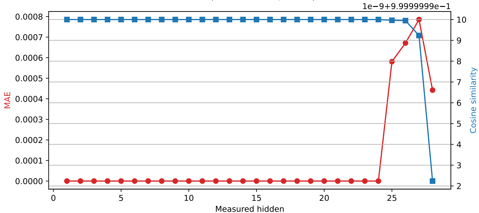
Qwen2.5-7B-Instruct | Quantized layer 24 | float32 → int16
