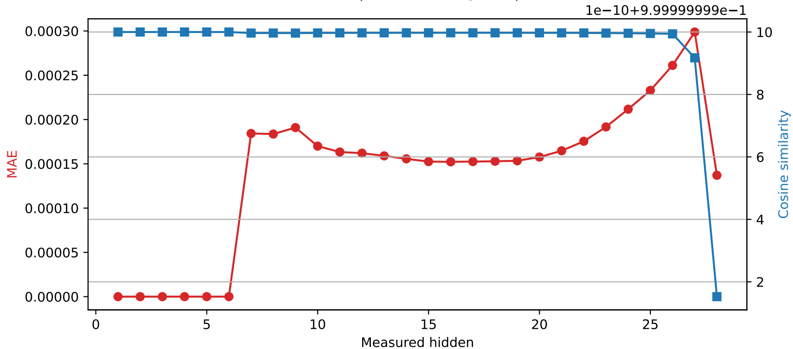
Qwen2.5-7B-Instruct | Quantized layer 6 | float32 \rightarrow int16
