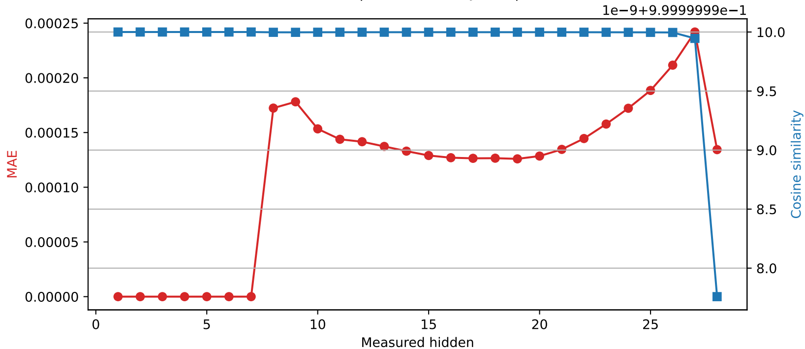
Qwen2.5-7B-Instruct | Quantized layer 7 | float32 \rightarrow int16
