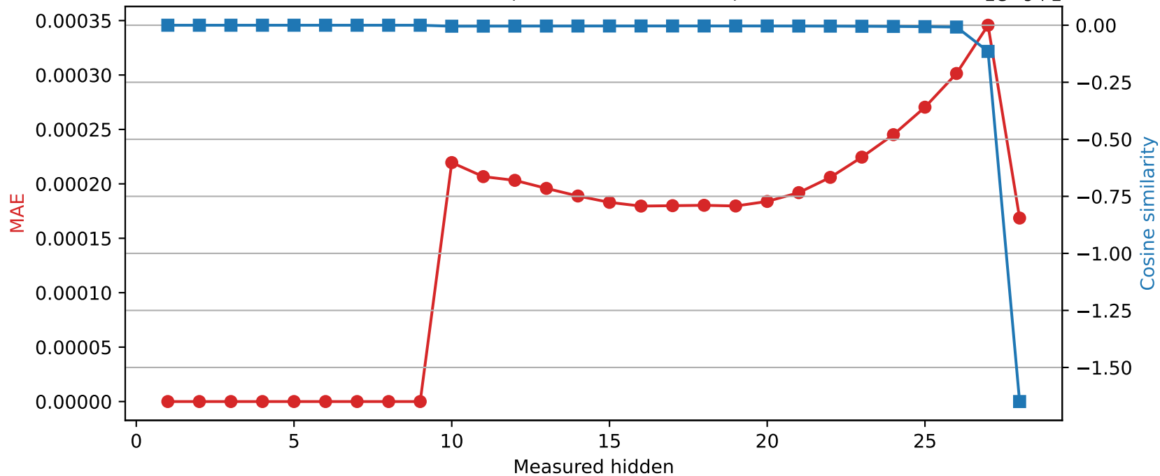
Qwen2.5-7B-Instruct | Quantized layer 9 | float32 → int16
