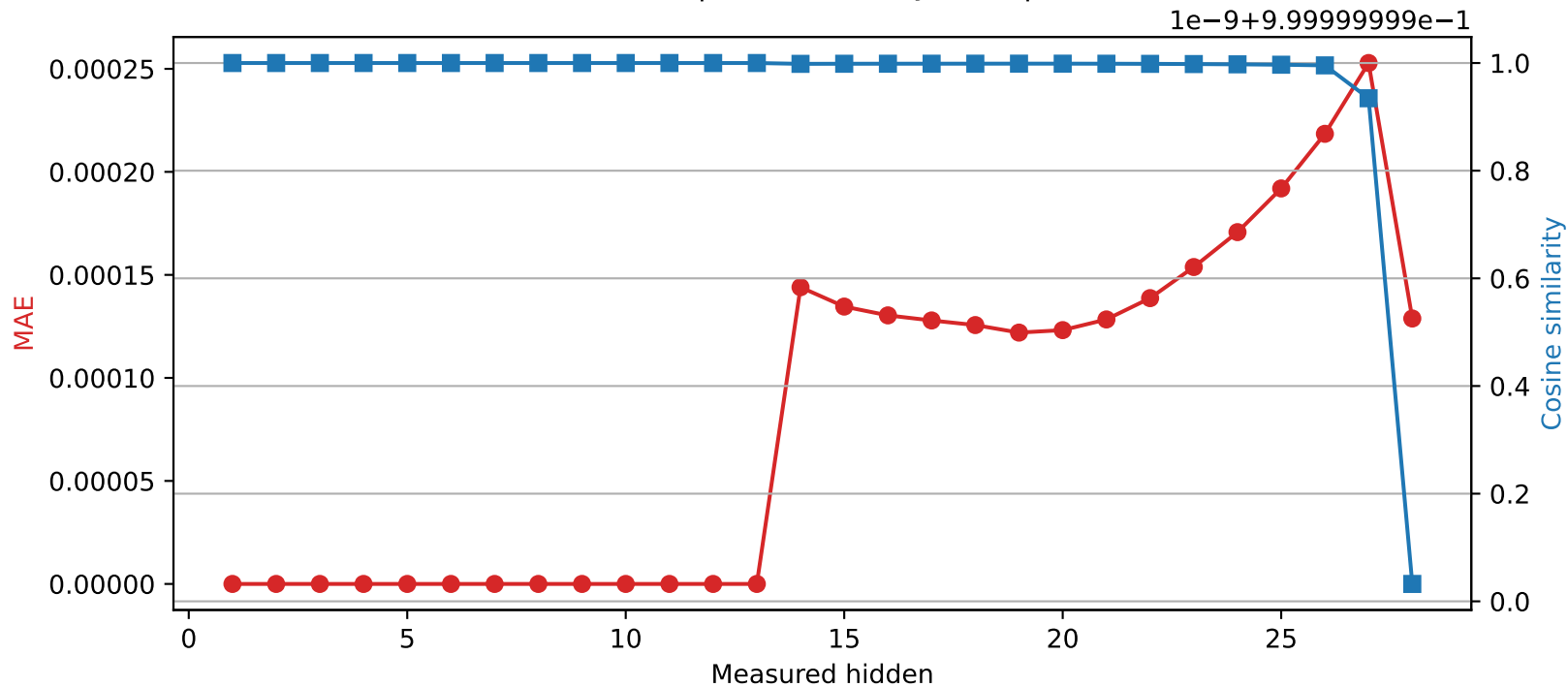
Qwen2.5-7B-Instruct | Quantized layer 13 | float32 → int16
