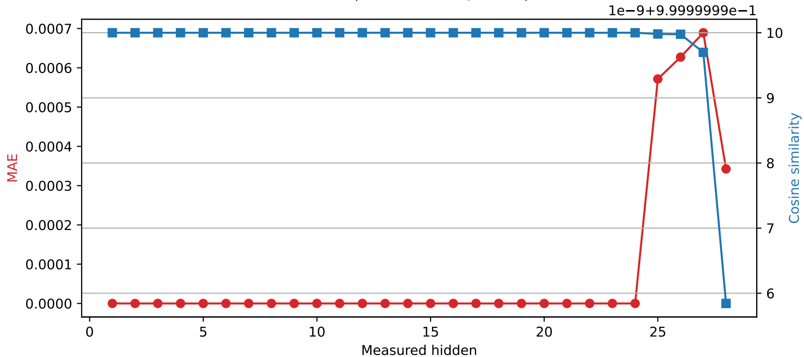
Qwen2.5-7B-Instruct | Quantized layer 24 | float64 \rightarrow int16
