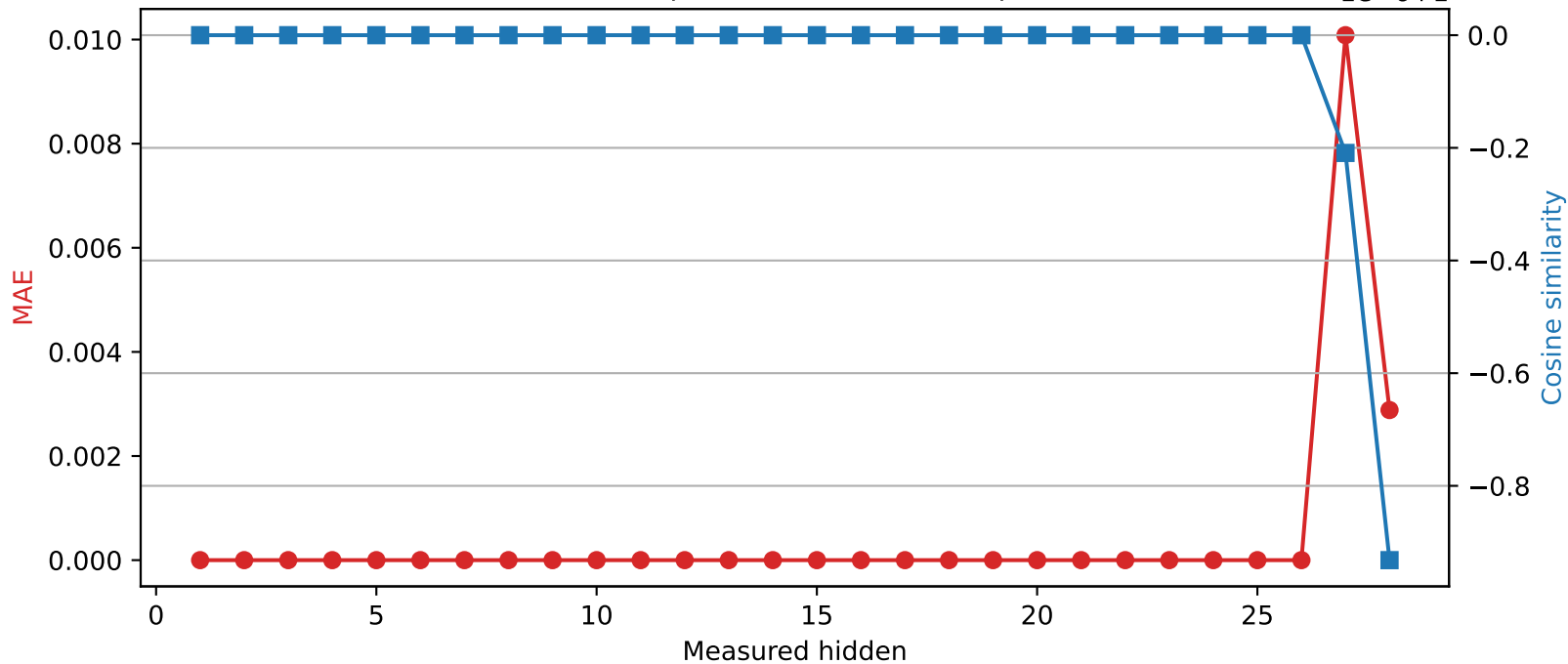
Qwen2.5-7B-Instruct | Quantized layer 26 | float64 → int16
