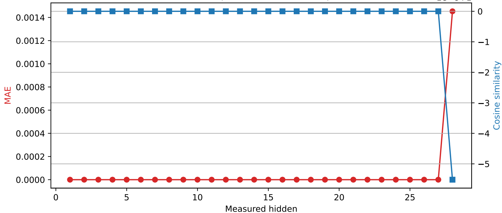
Qwen2.5-7B-Instruct | Quantized layer 27 | float64 → int16
