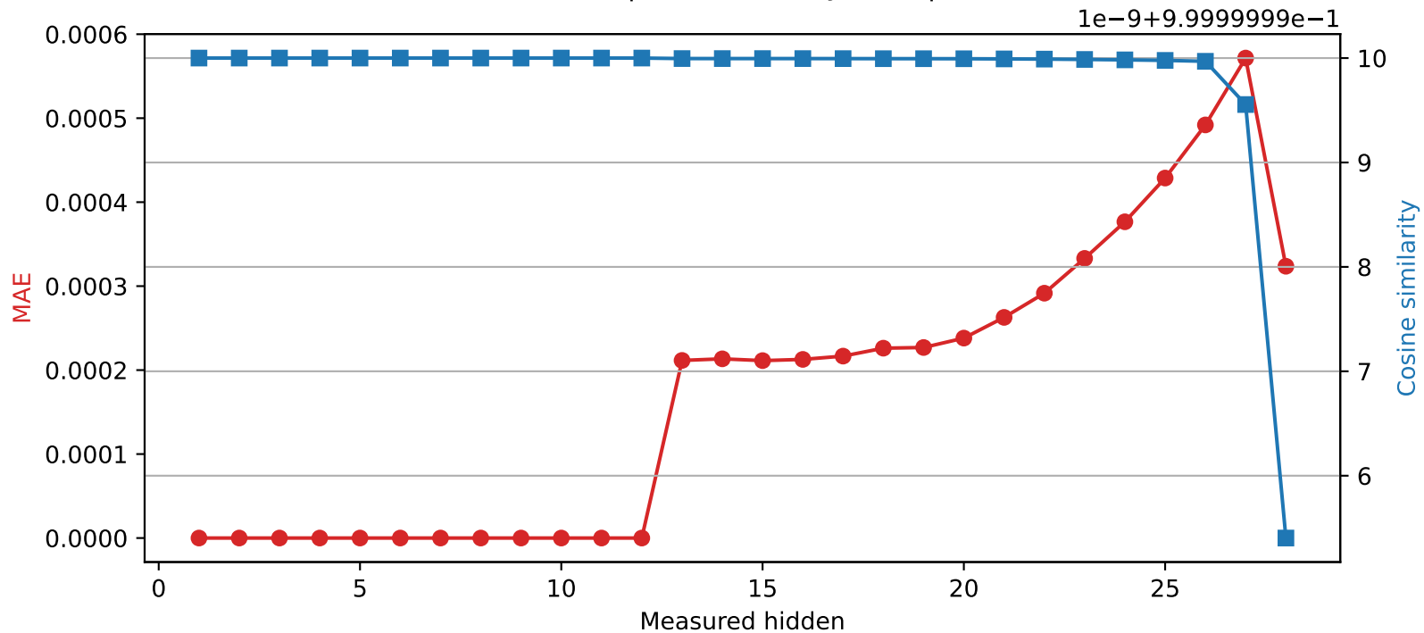
Qwen2.5-7B-Instruct | Quantized layer 12 | float64 → int16
