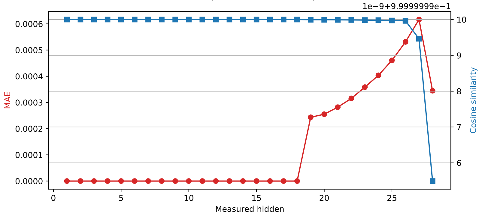
Qwen2.5-7B-Instruct | Quantized layer 18 | float64 → int16
