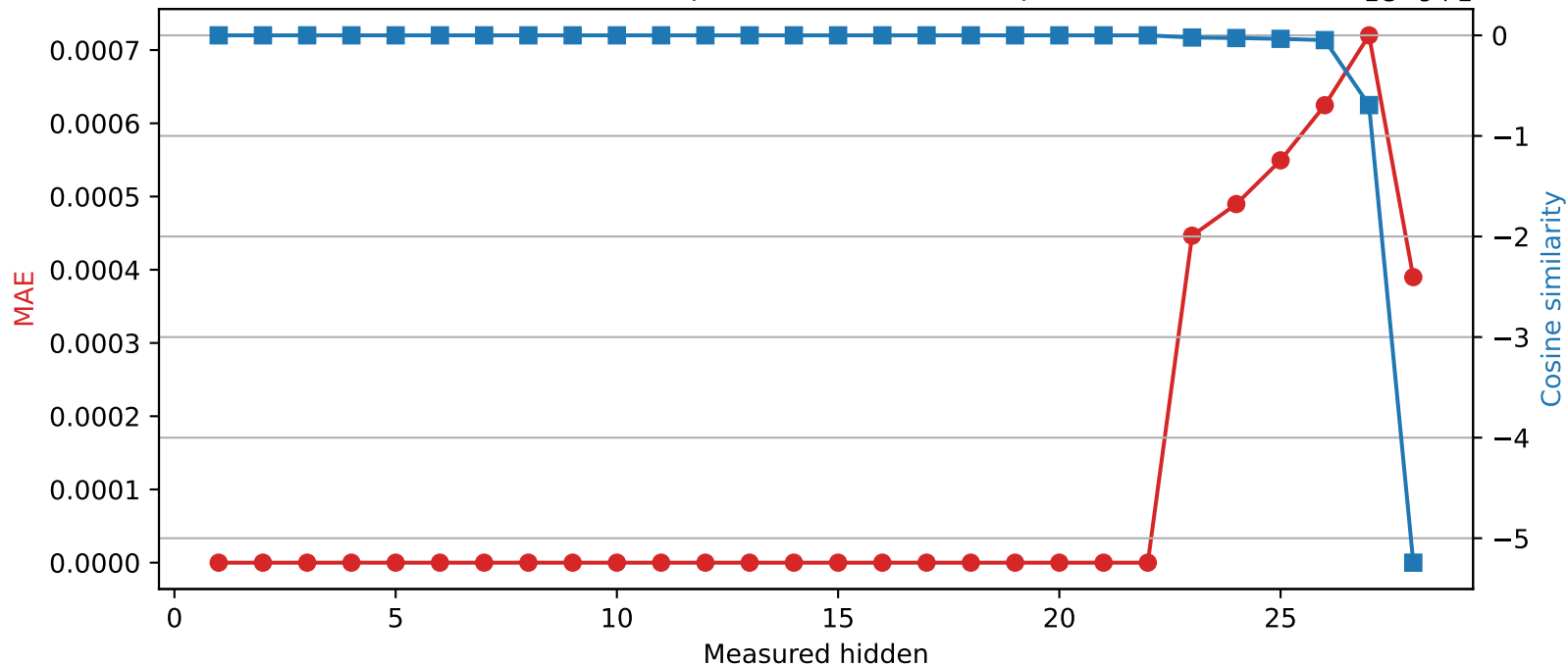
Qwen2.5-7B-Instruct | Quantized layer 22 | float64 → int16
