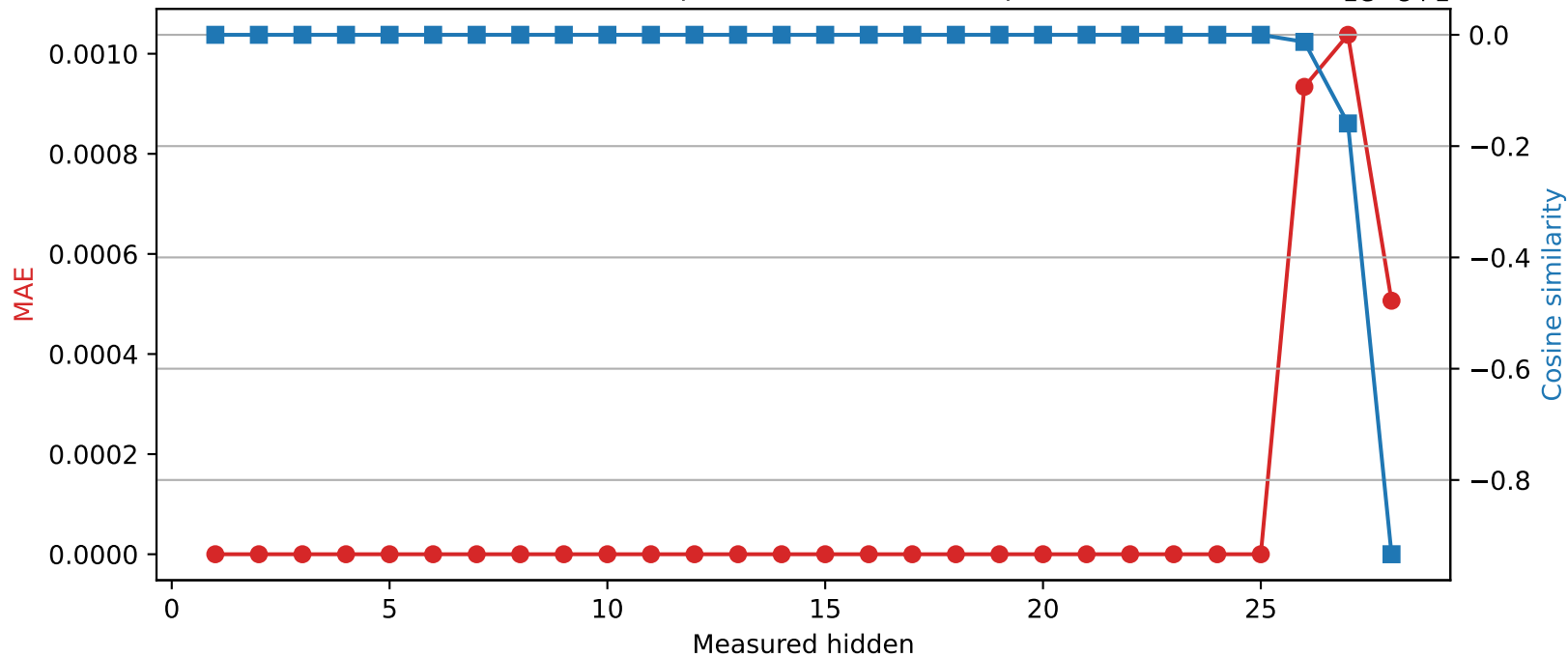
Qwen2.5-7B-Instruct | Quantized layer 25 | float64 → int16
