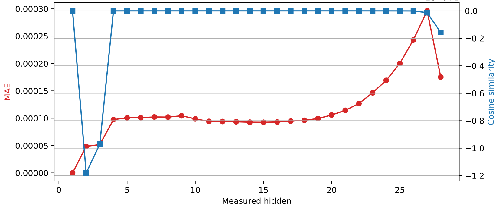
Qwen2.5-7B-Instruct | Quantized layer 1 | float64 → int16
