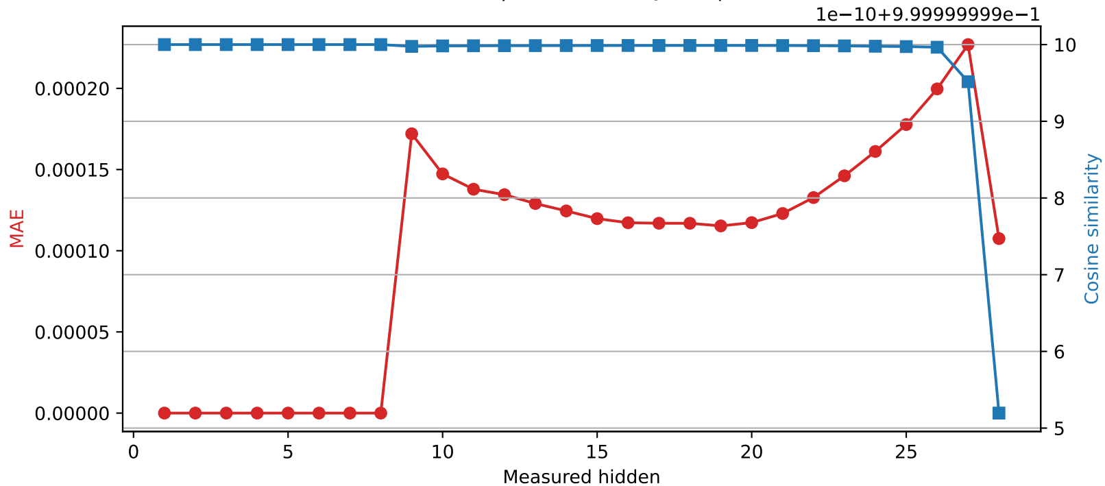
Qwen2.5-7B-Instruct | Quantized layer 8 | float64 → int16
