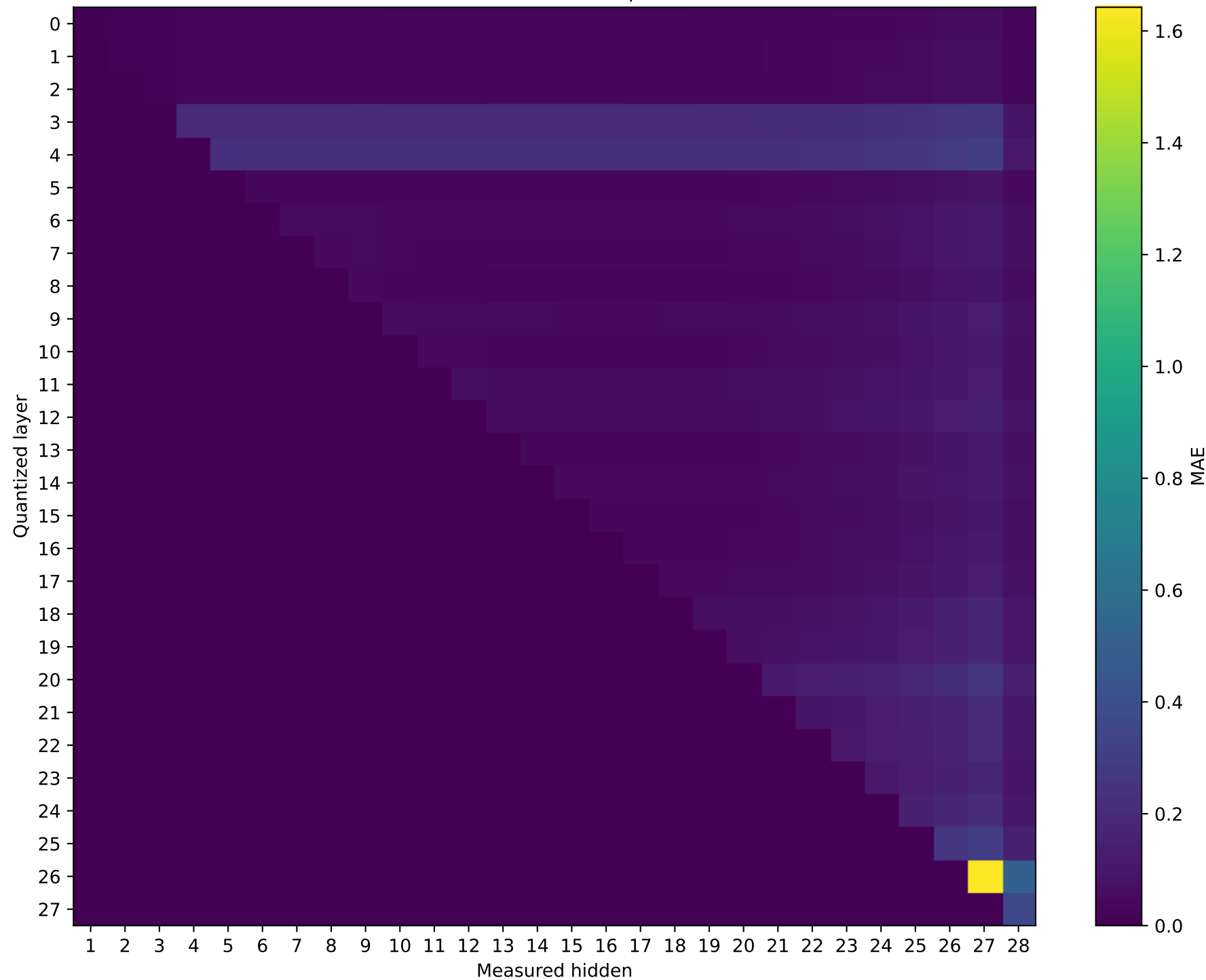
Model: Qwen2.5-7B-Instruct | float16 → int8
