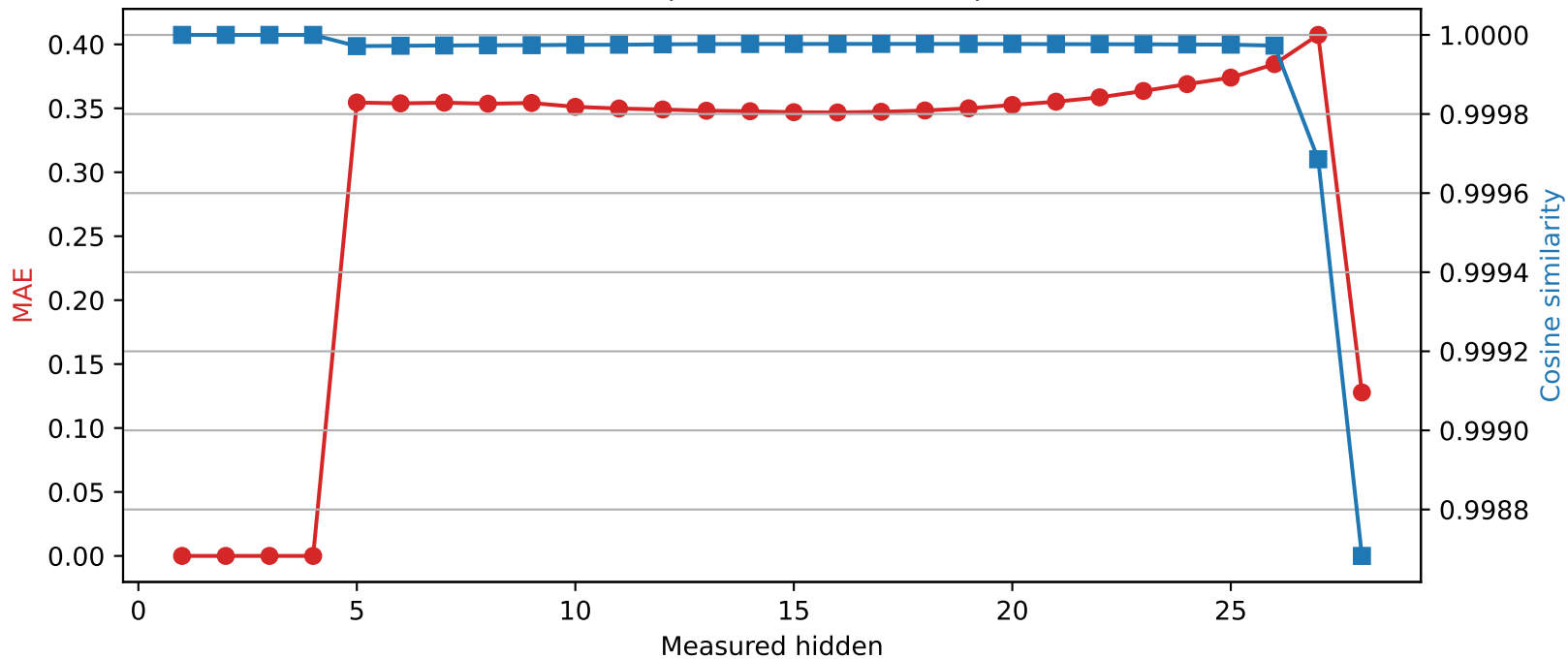
Qwen2.5-7B-Instruct | Quantized layer 4 | float16 \rightarrow int8
