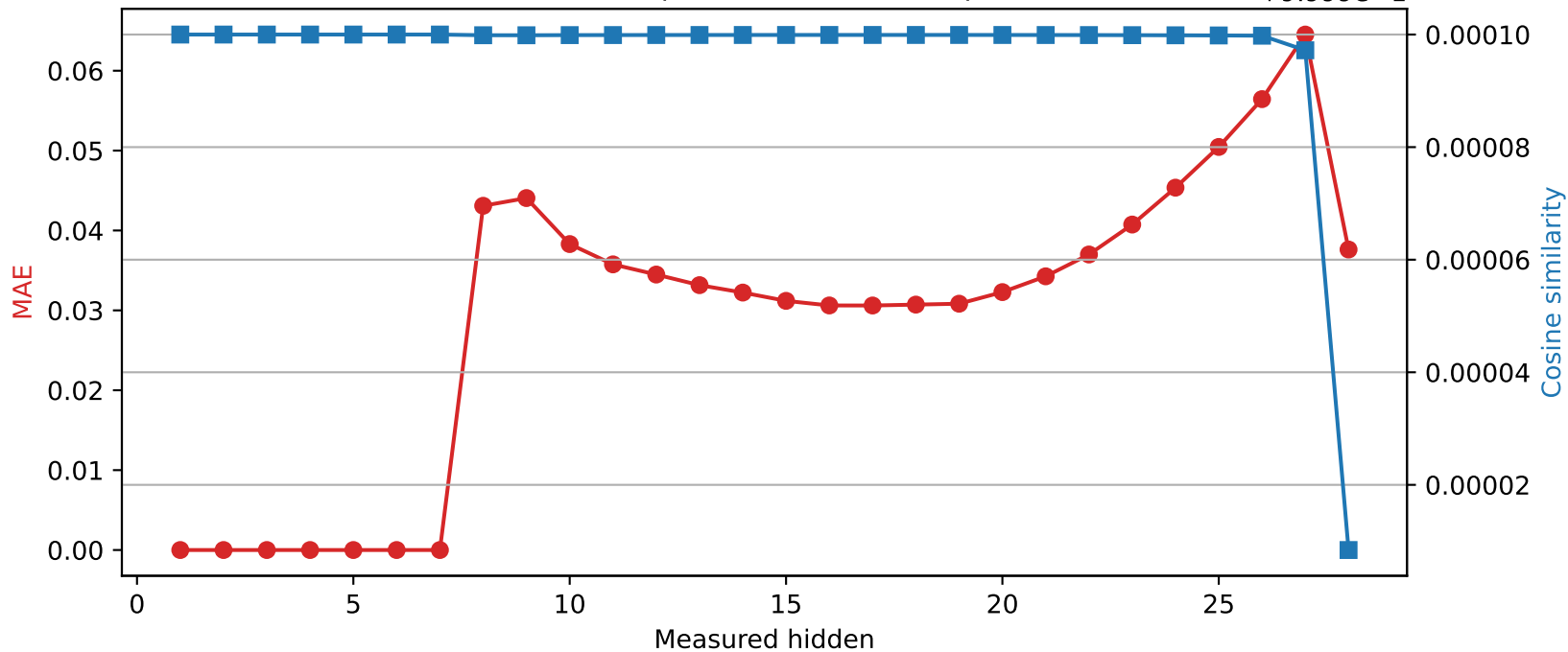
Qwen2.5-7B-Instruct | Quantized layer 7 | float16 → int8
