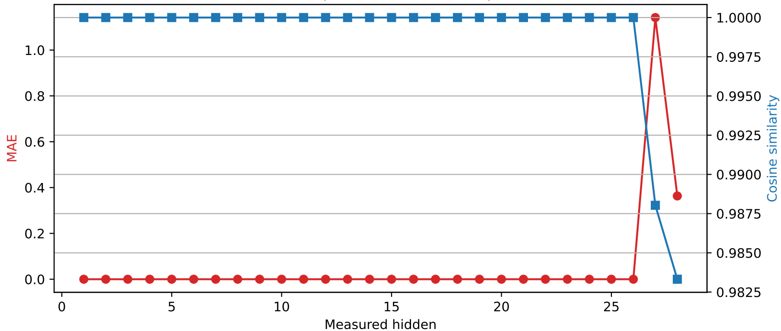
Qwen2.5-7B-Instruct | Quantized layer 26 | float16 \rightarrow int8
