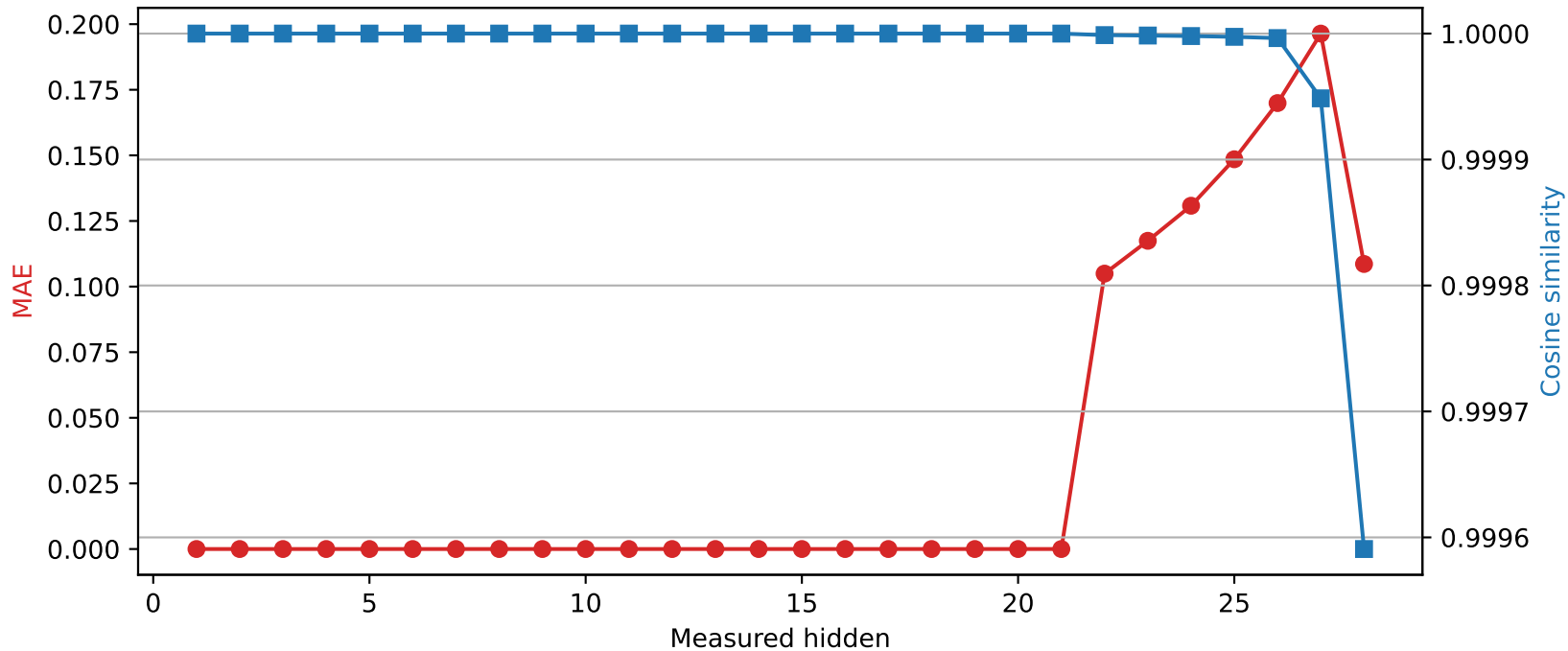
Qwen2.5-7B-Instruct | Quantized layer 21 | float16 → int8
