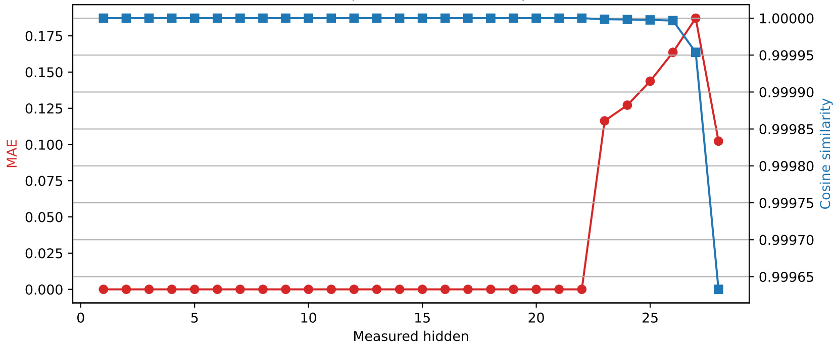
Qwen2.5-7B-Instruct | Quantized layer 22 | float16 → int8
