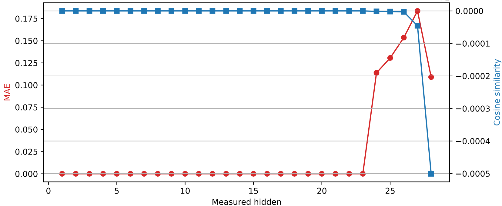
Qwen2.5-7B-Instruct | Quantized layer 23 | float16 \rightarrow int8
