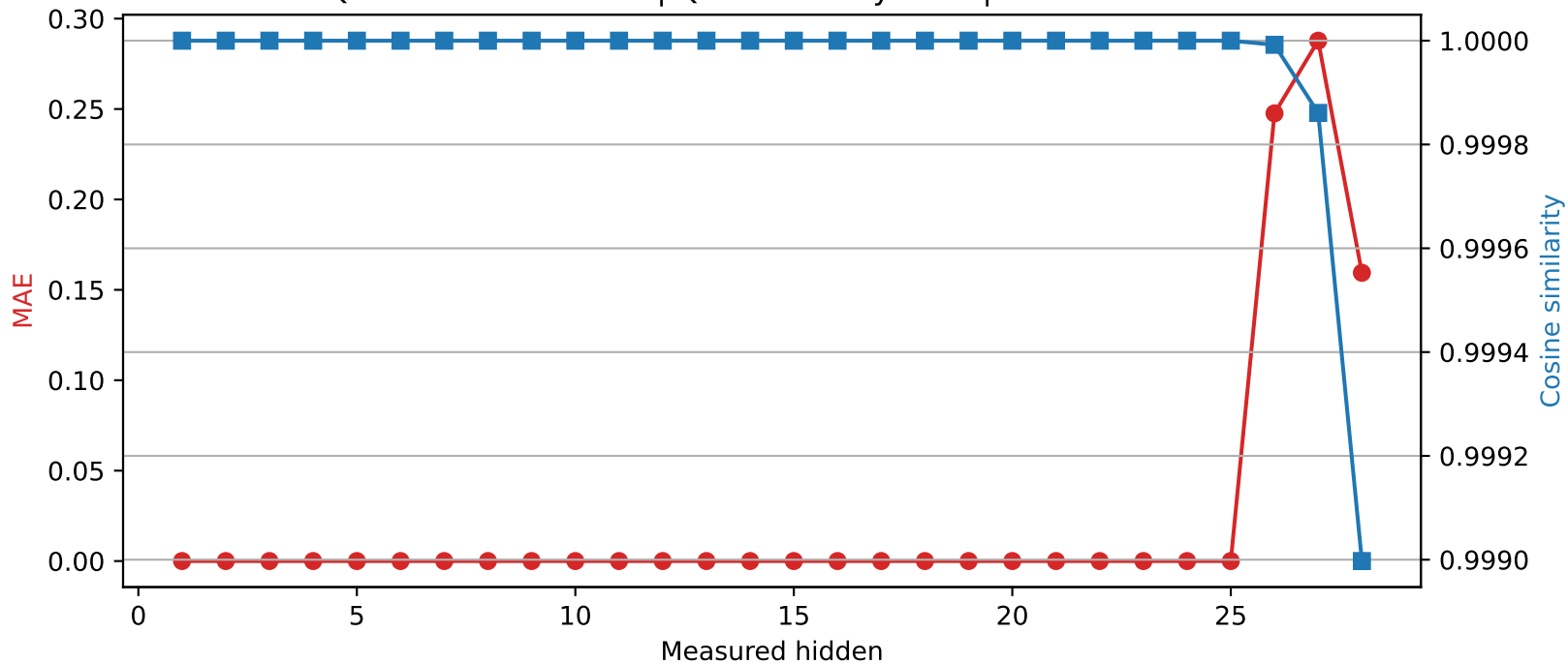
Qwen2.5-7B-Instruct | Quantized layer 25 | float16 → int8
