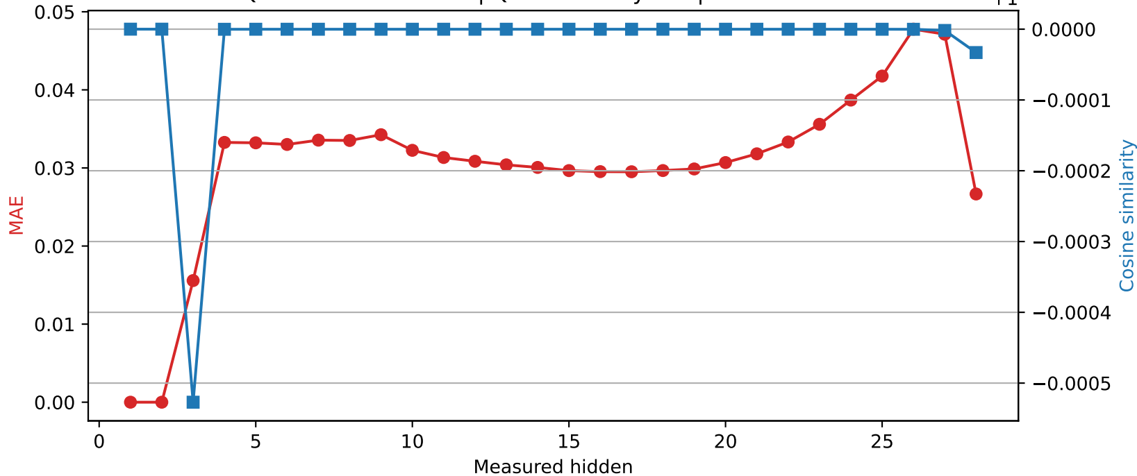
Qwen2.5-7B-Instruct | Quantized layer 2 | float32 → int8
