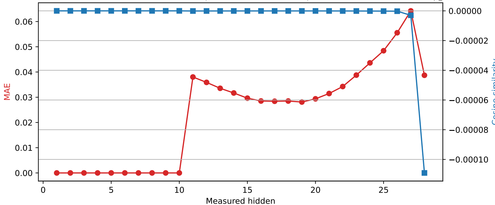
Qwen2.5-7B-Instruct | Quantized layer 10 | float32 → int8
