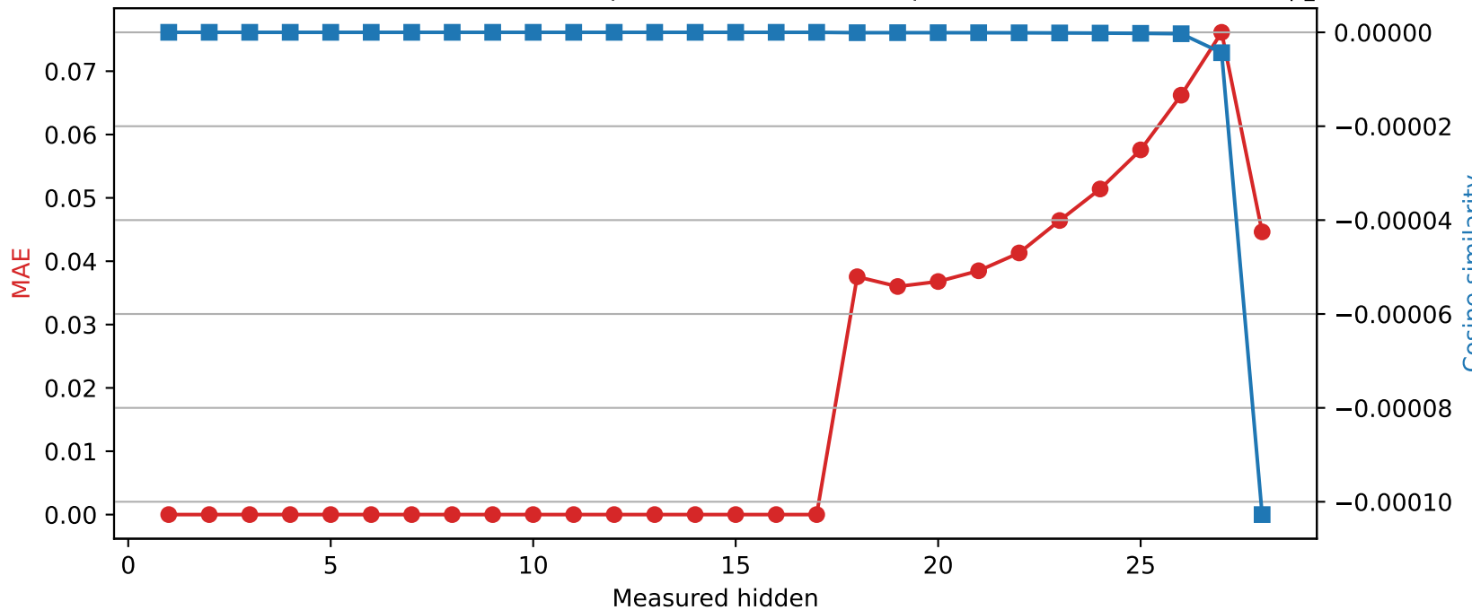
Qwen2.5-7B-Instruct | Quantized layer 17 | float32 → int8
