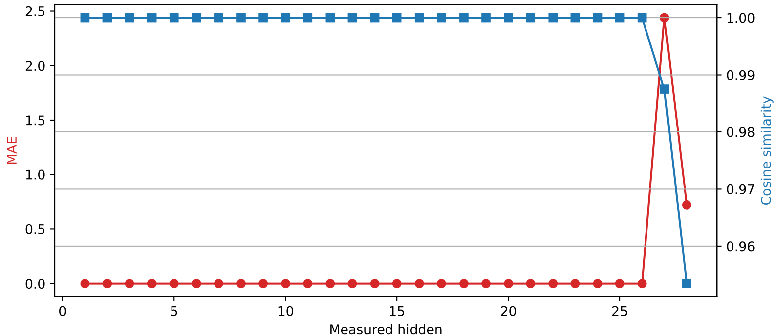
Qwen2.5-7B-Instruct | Quantized layer 26 | float32 \rightarrow int8
