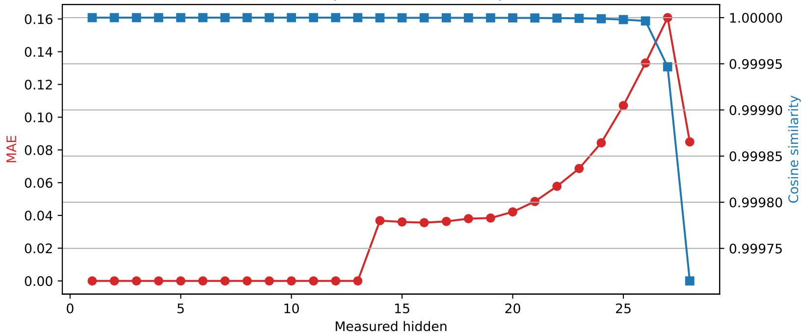
Qwen2.5-7B-Instruct | Quantized layer 13 | float32 \rightarrow int8
