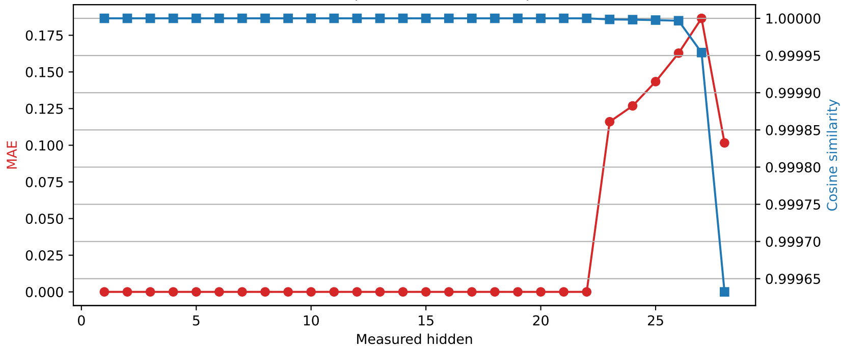
Qwen2.5-7B-Instruct | Quantized layer 22 | float32 → int8
