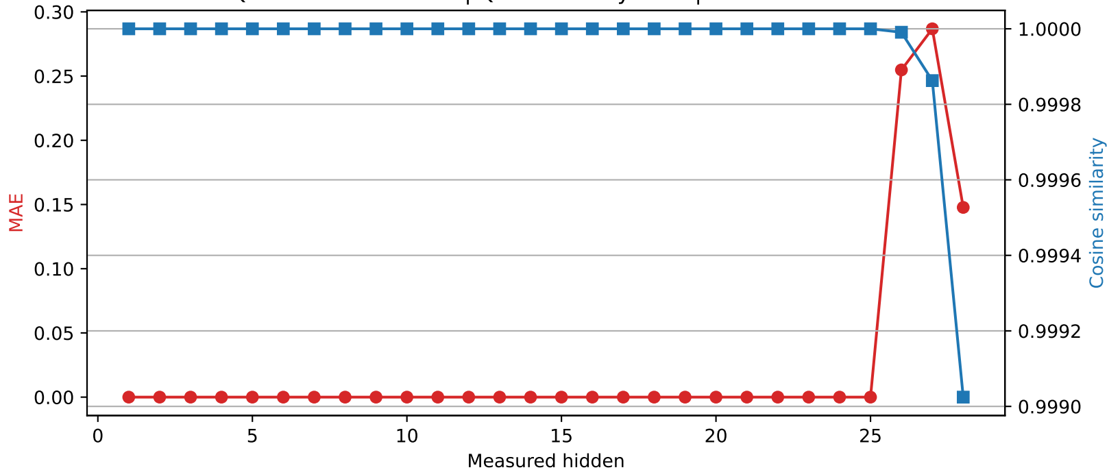
Qwen2.5-7B-Instruct | Quantized layer 25 | float32 \rightarrow int8
