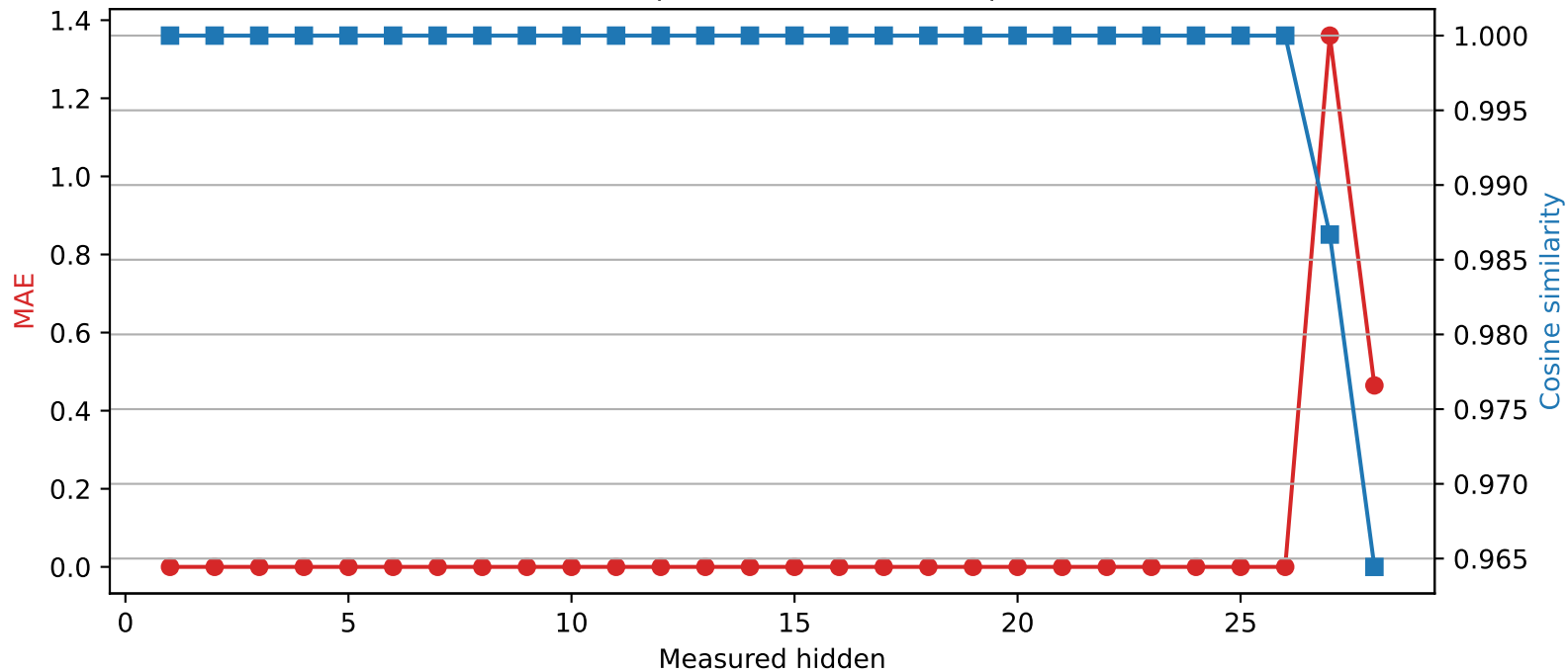
Qwen2.5-7B-Instruct | Quantized layer 26 | float32 → int8
