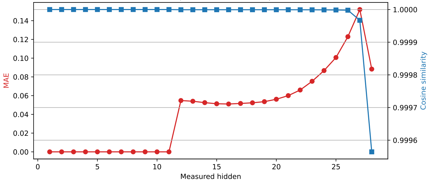
Qwen2.5-7B-Instruct | Quantized layer 11 | float32 \rightarrow int8
