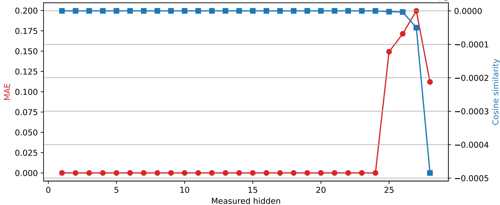
Qwen2.5-7B-Instruct | Quantized layer 24 | float32 → int8
